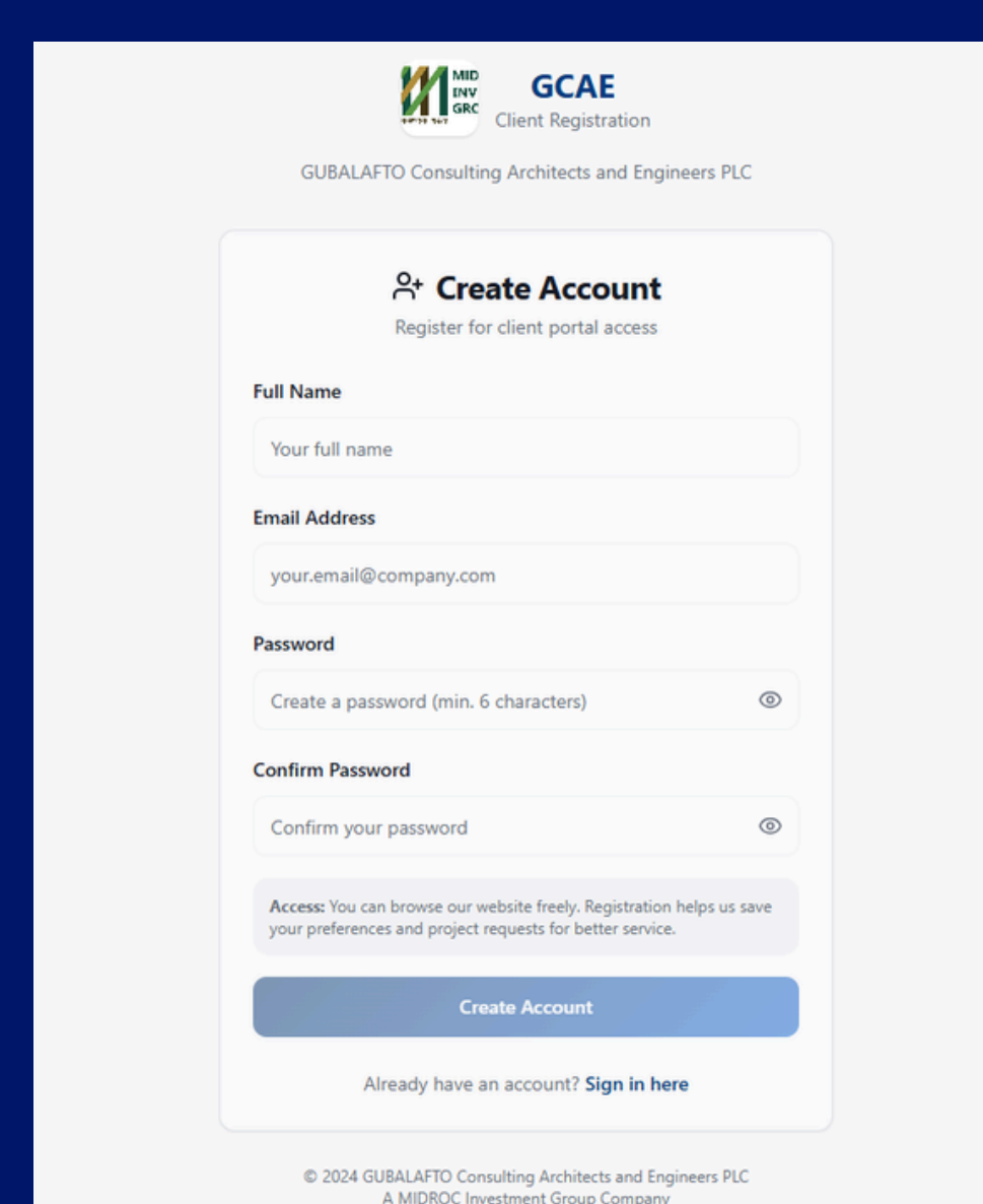
REGISTER/SIGN-UP
