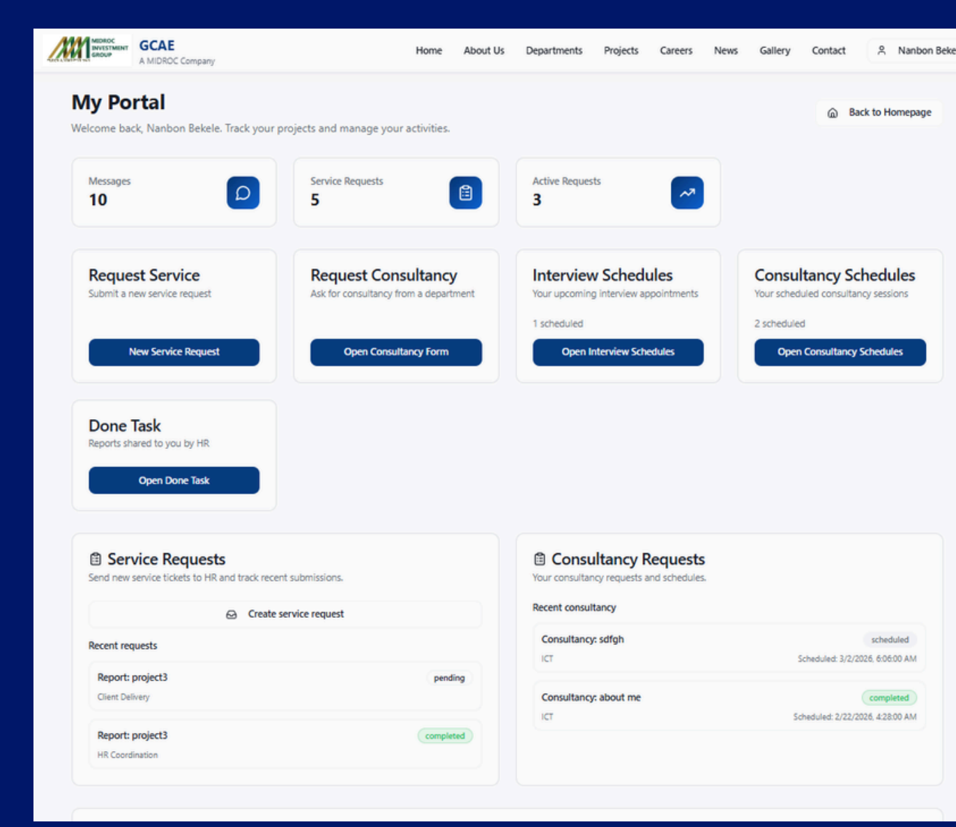
CLIENT DASHBOARD
