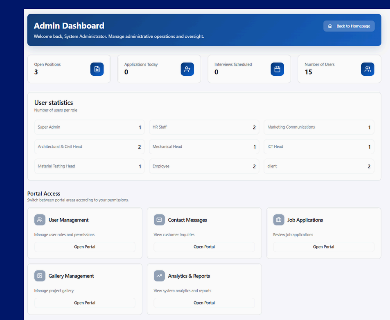
ADMIN DASHBOARD
