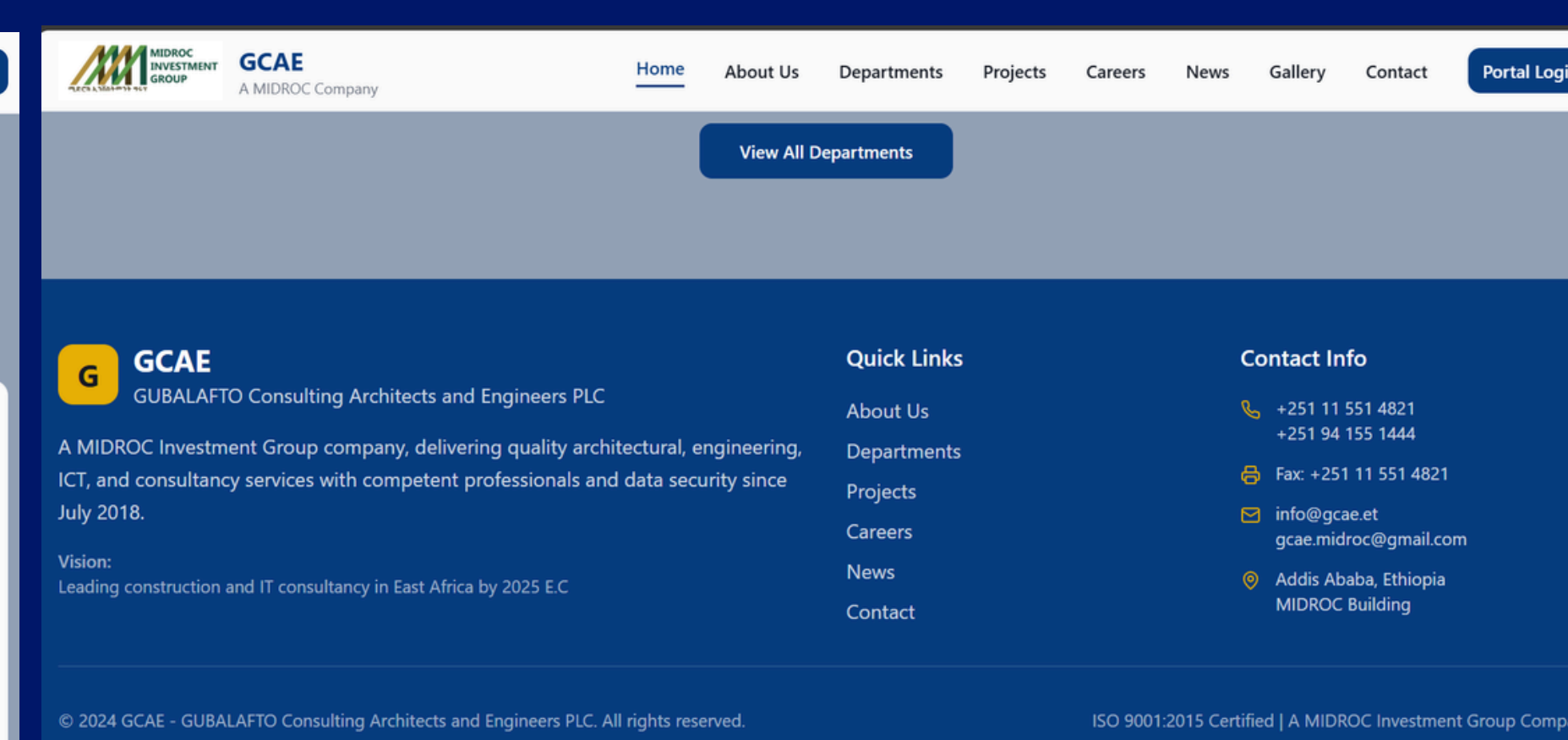
CONT...HOMEPAGE
