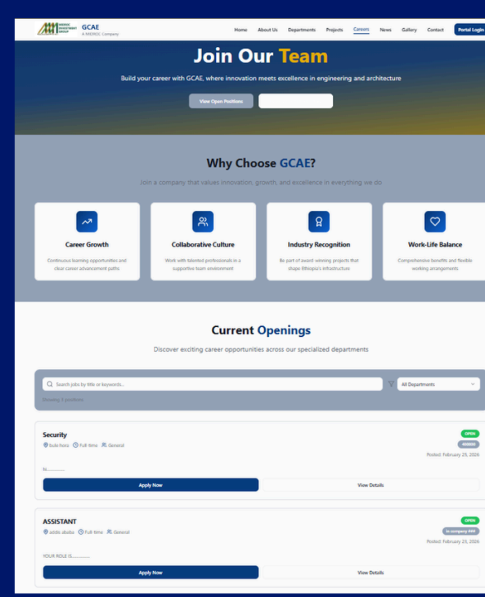
OPEN JOB
