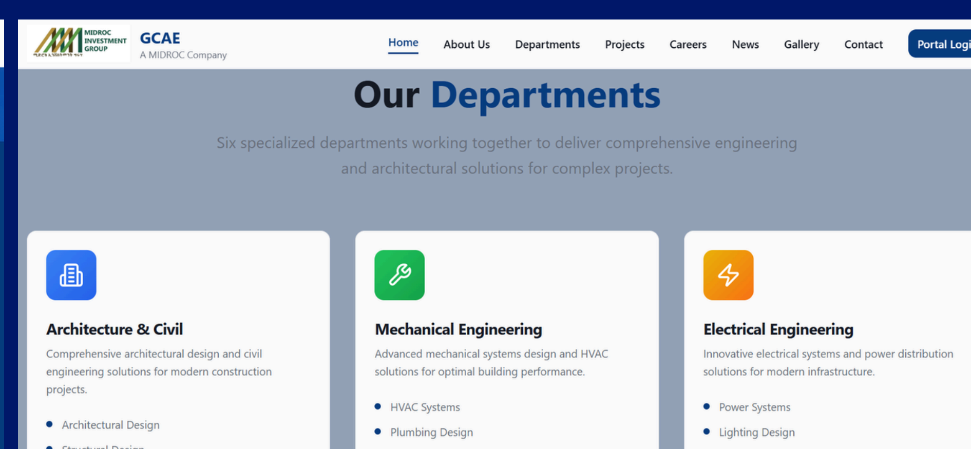
CONT...HOMEPAGE
