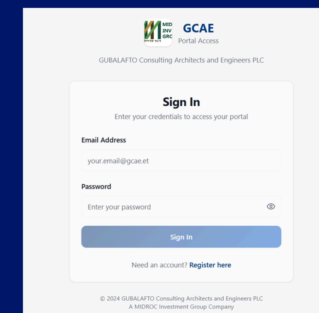
LOGIN/SIGN IN
