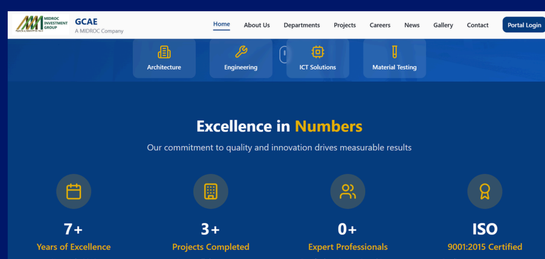
CONT...HOMEPAGE
