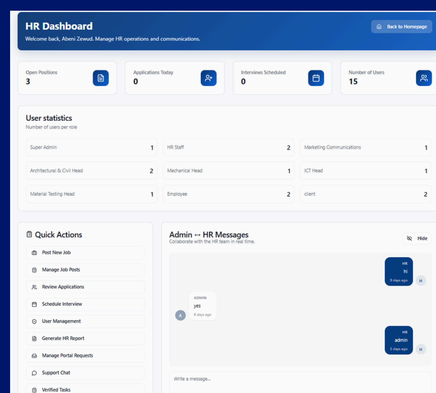
HR-DAHSBOARD
