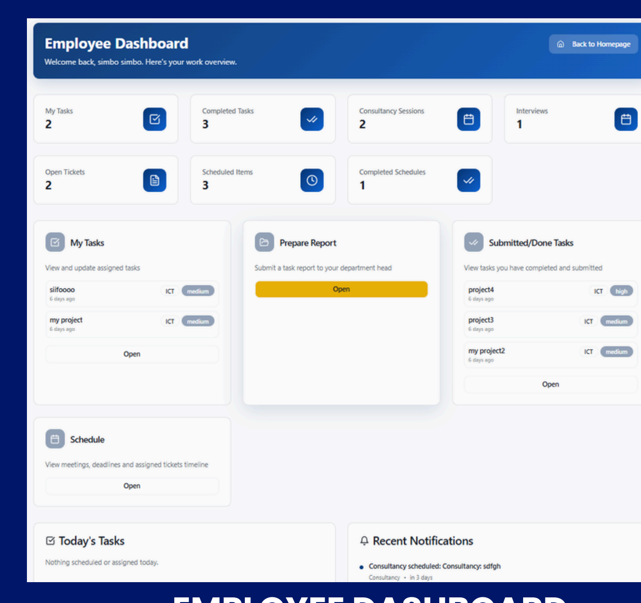
EMPLOYEE DASHBOARD
